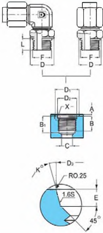
Detail X
